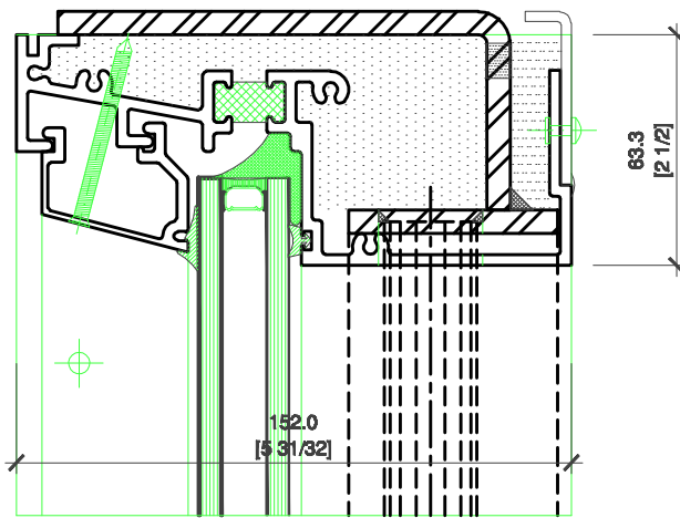
5 SLIDER DETAIL
