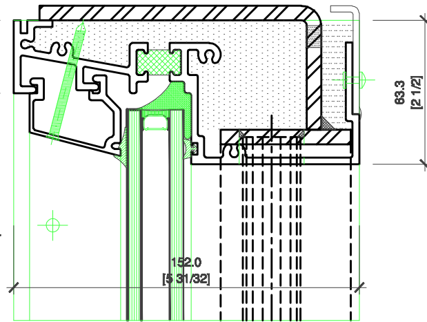
5 SLIDER DETAIL
