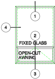
TYPICAL ELEVATION TYPE OF SECURITY GLASS - TO ARCHITECT'S SELECTION
