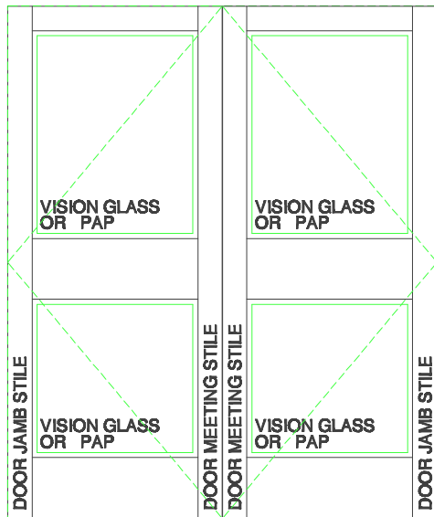
TYPICAL ELEVATION TYPE OF GLASS AND PANEL - TO ARCHITECT'S SELECTION
